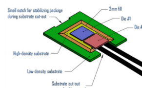
PC7.1.1: FHE Interposer for heterogeneous integration of a high-density Fiber Optic Multi-chip module led by Lockheed Martin
