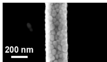
PC8.8.2: Ultra-Fine Resolution Printing of Circuit Components led by Northeastern University.
