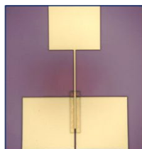
PC8.8.2: Ultra-Fine Resolution Printing of Circuit Components led by Northeastern University.
