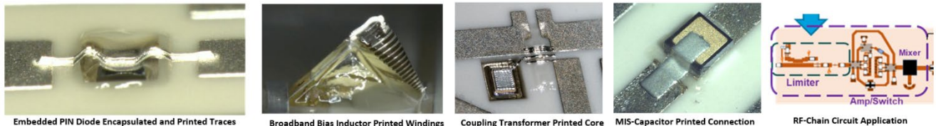
PC6.2: Reliability Validation and Sustainment of Direct-Write Printed RF Devices led by Lockheed Martin.
